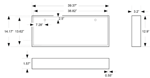
Figure B. Model XL-84B, rear view
