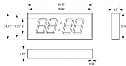
Figure A. Model XL-84B, front view
