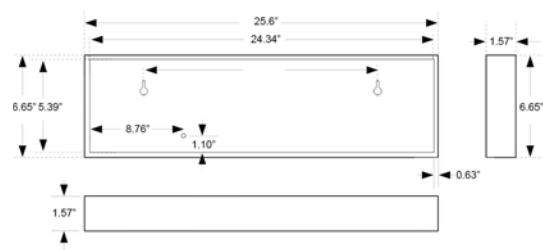
Figure B. Model XL-46R-100, rear view
