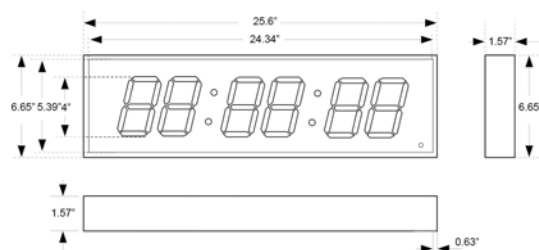
Figure A. Model XL-46R-100, front view
