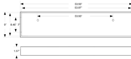
Figure B. Model XL-79, rear view
