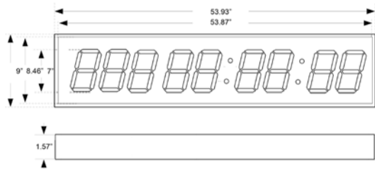
Figure A. Model XL-79, front view
